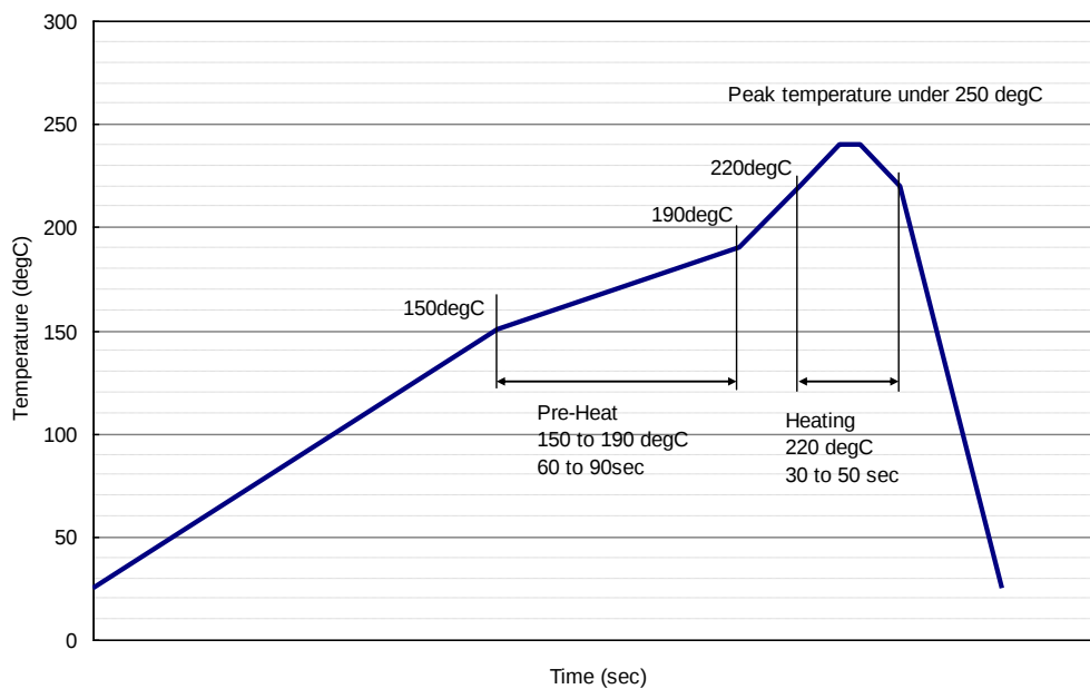
Figure 6. 推奨リフロー条件 Recommendation soldering conditions
