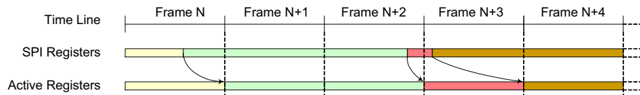
Figure 18. Frame Synchronization of Configurations (no freezing)
