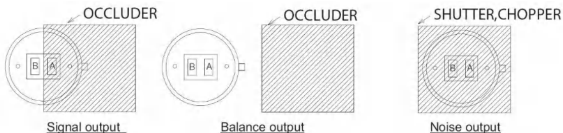
Figure 2 - Occluder Position
