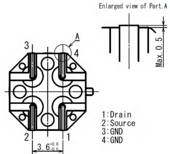
Figure 7 - Bottom View
