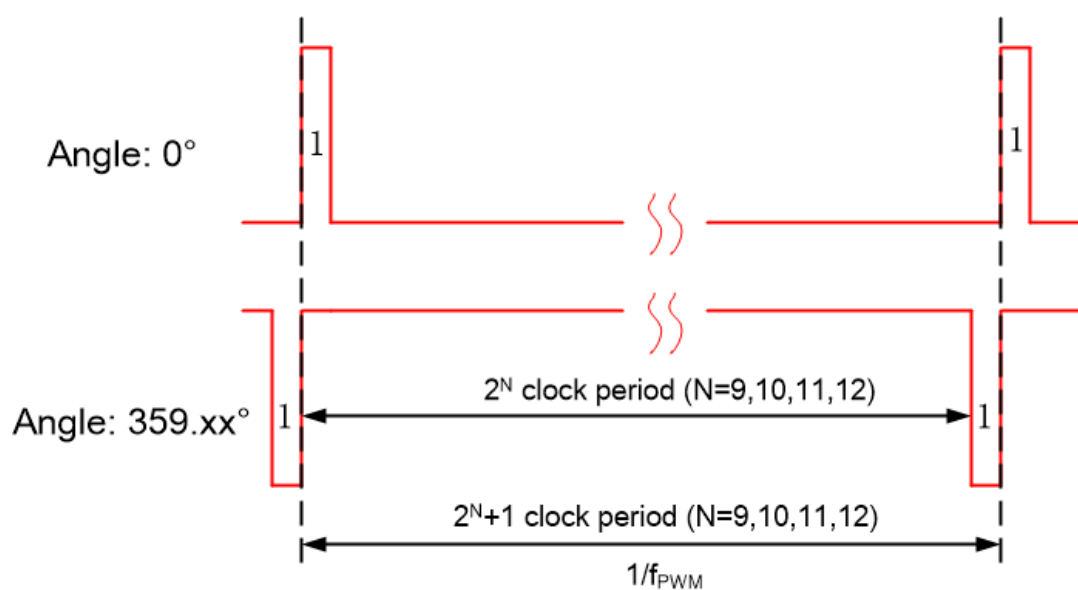
Figure 9: PWM Output
