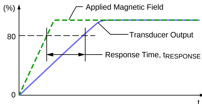
Figure 3: Response Time definition
