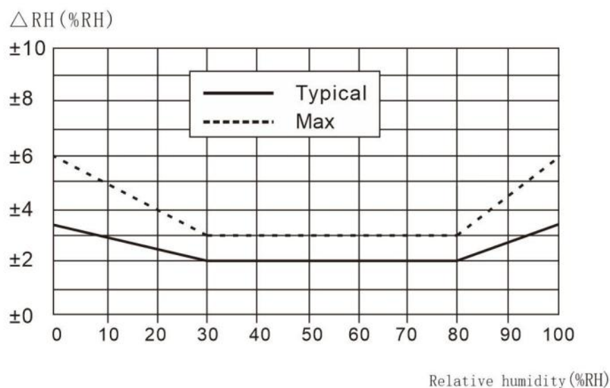
Figure 2. Typical and maximum humidity errors
