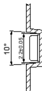
Figure 7: Carrier Tape
