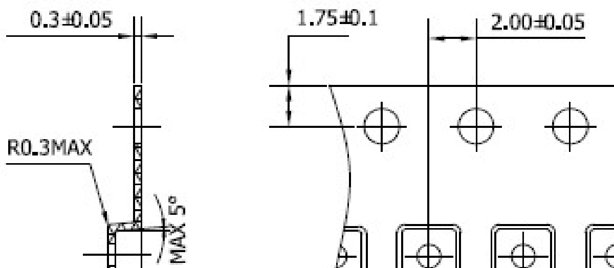
Figure 10 Tape and reel dimension in mm
