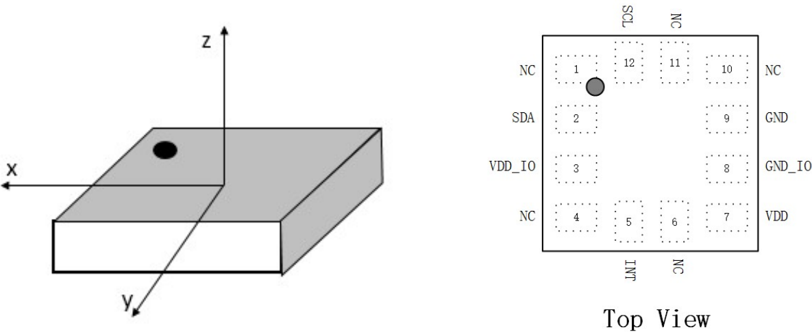
Figure 2 Pin description
