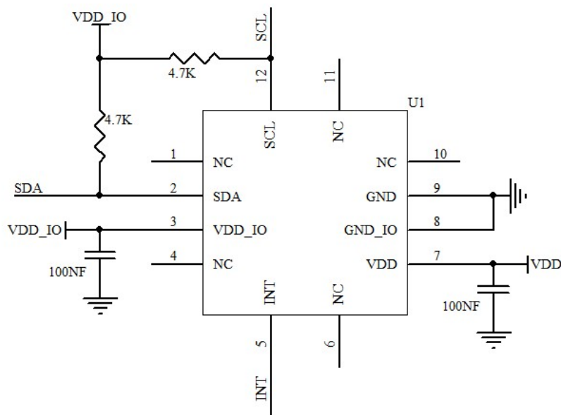
Figure 7 da218G I2C electrical connect
