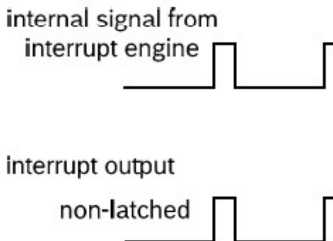
Figure 6 Interrupt mode
