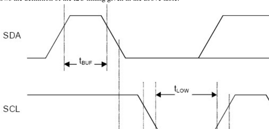
Figure 3 I2C Slave timing diagram
