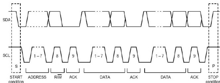
Figure 4 I2C Protocol
