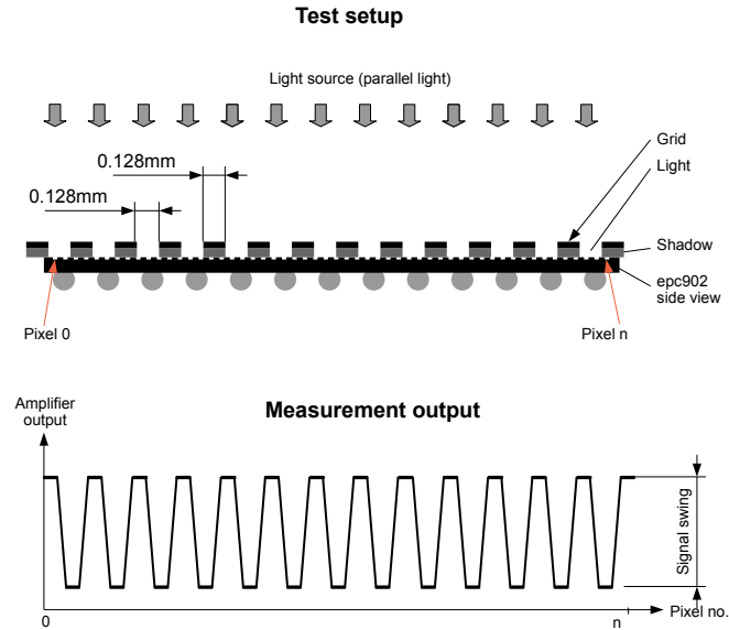
Figure 5: Modulation measurement
