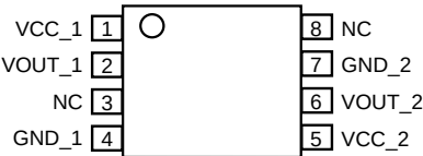
LE-8 Package Pinout (dual die)
