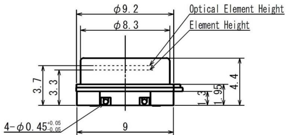
Figure 8 - Side View
