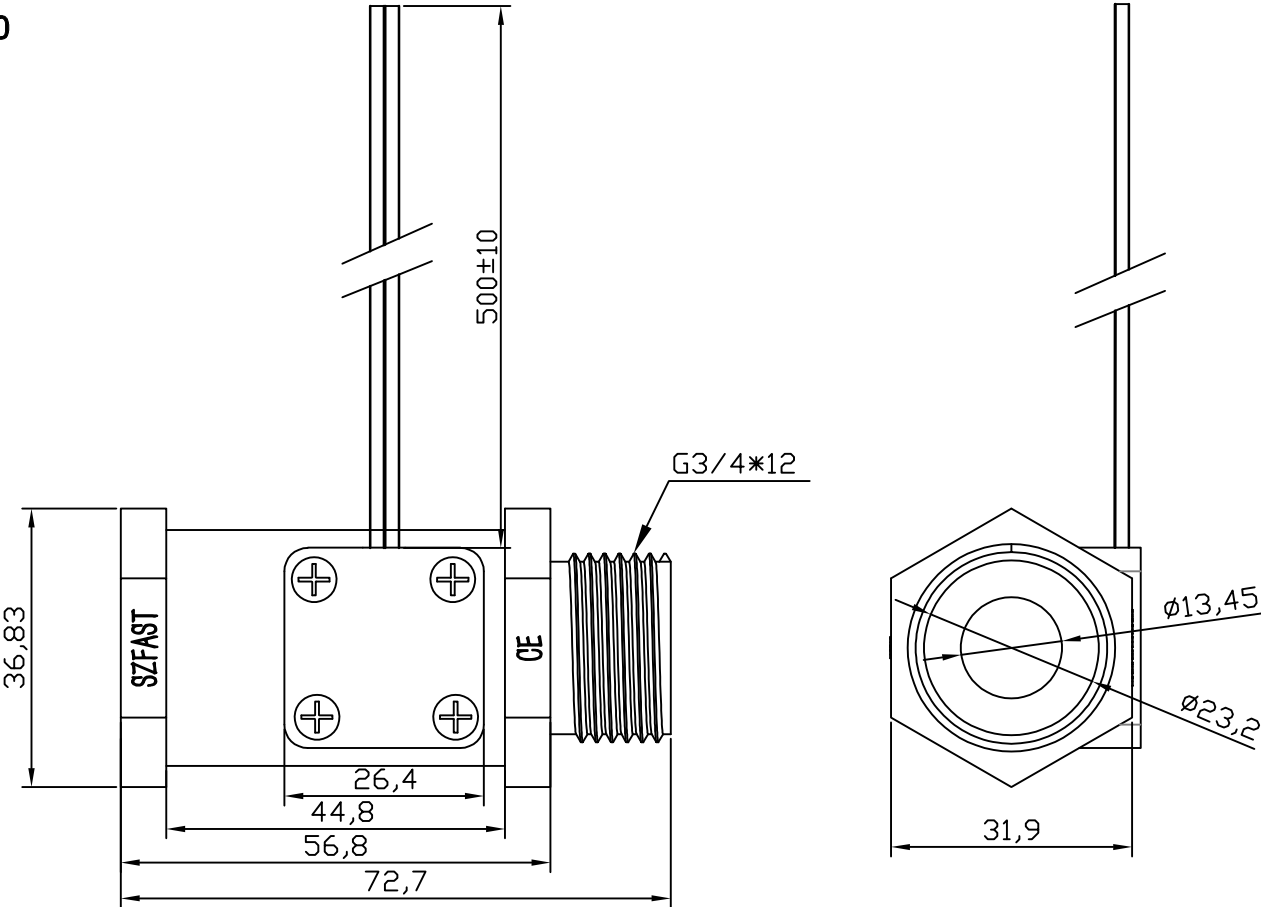
FHS-2PV-1T30-DN20
