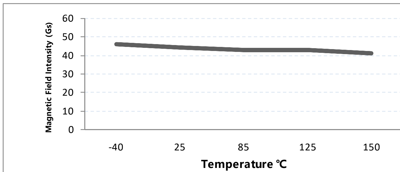
Figure.8 Magnetic Characteristics vs. Temperature (BHYST)
