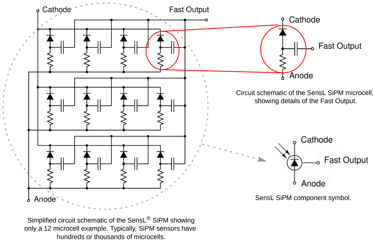
Figure 2. Circuit Schematic
