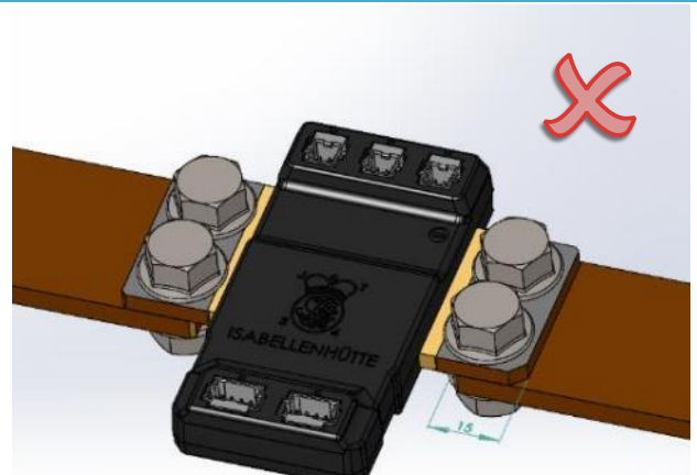
Figure 16: Incorrect mounting 15mm overlap
