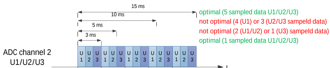
Figure 5: Example with three channel on ADC2
