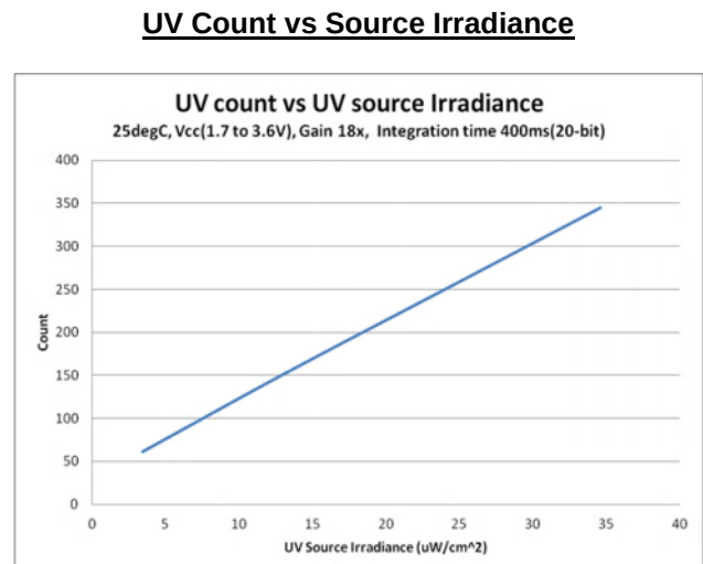
Figure 4.4 UV Count vs Source Irradiance
