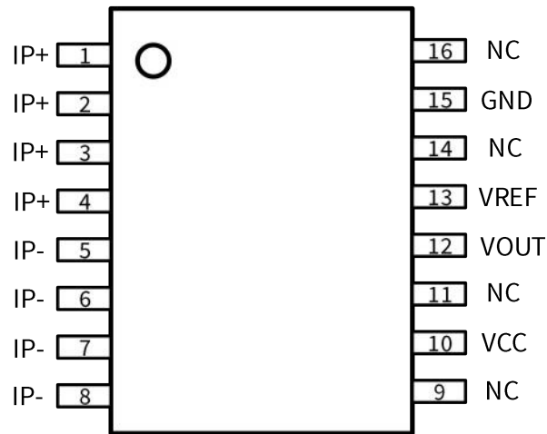
Figure 1.1 NSM2013 Package
