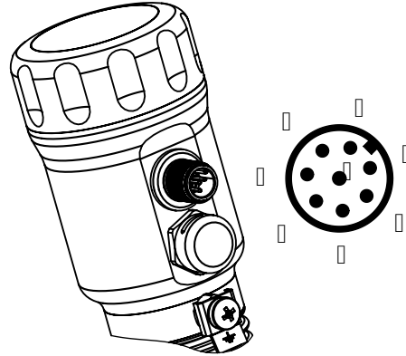
M12 round connector, 8-pin
