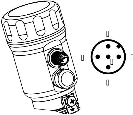
M12 round connector, 5-pin
