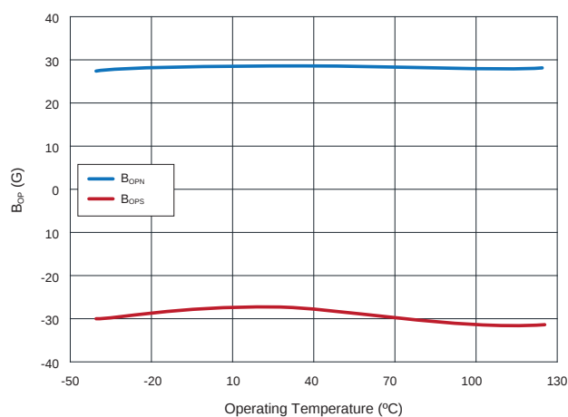
12.6 RR132-1B12-551 / 552 B_{OPN} (Blue) and B_{OPS} (Red) vs. Operating Temperature at V_{DD}=3.0 V
