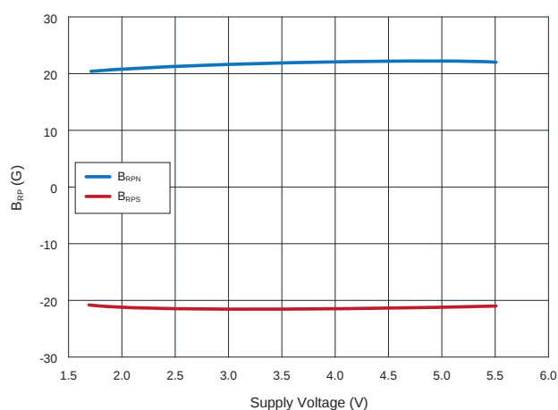
12.5 RR132-1B12-551 / 552 B_{RPN} (Blue) and B_{RPS} (Red) vs. Supply Voltage at +25°C
