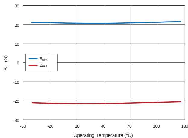
12.7 RR132-1B12-551 / 552 B_{RPN} (Blue) and B_{RPS} (Red) vs. Operating Temperature at V_{DD}=3.0 V
