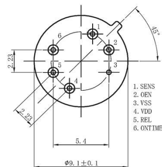
底视 Base view
