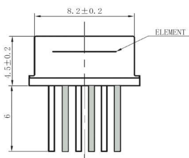
侧视 Side view
