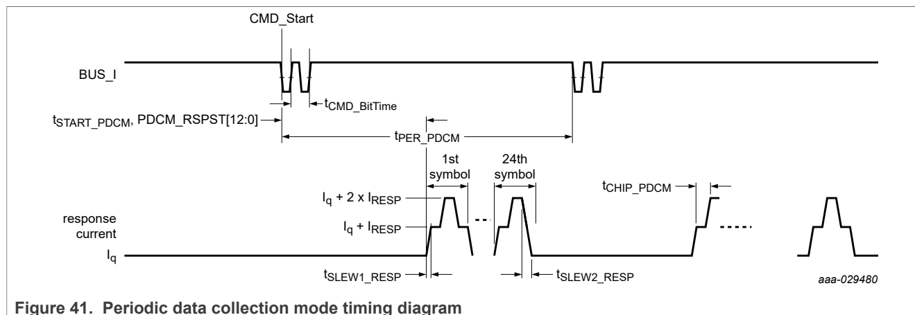
Figure 41. Periodic data collection mode timing diagram
