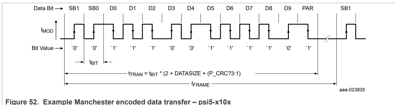
Figure 52. Example Manchester encoded data transfer – psi5-x10x
