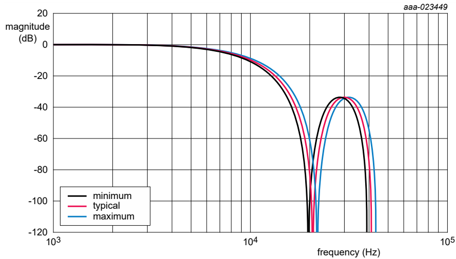
Figure 14. Sinc filter response
