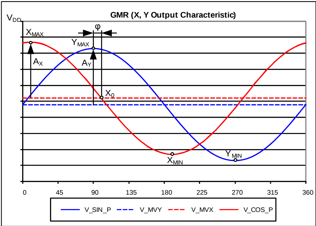
Figure 15 GMR sensor single-ended output signals
