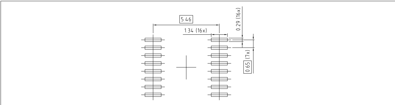
Figure 23 Footprint
