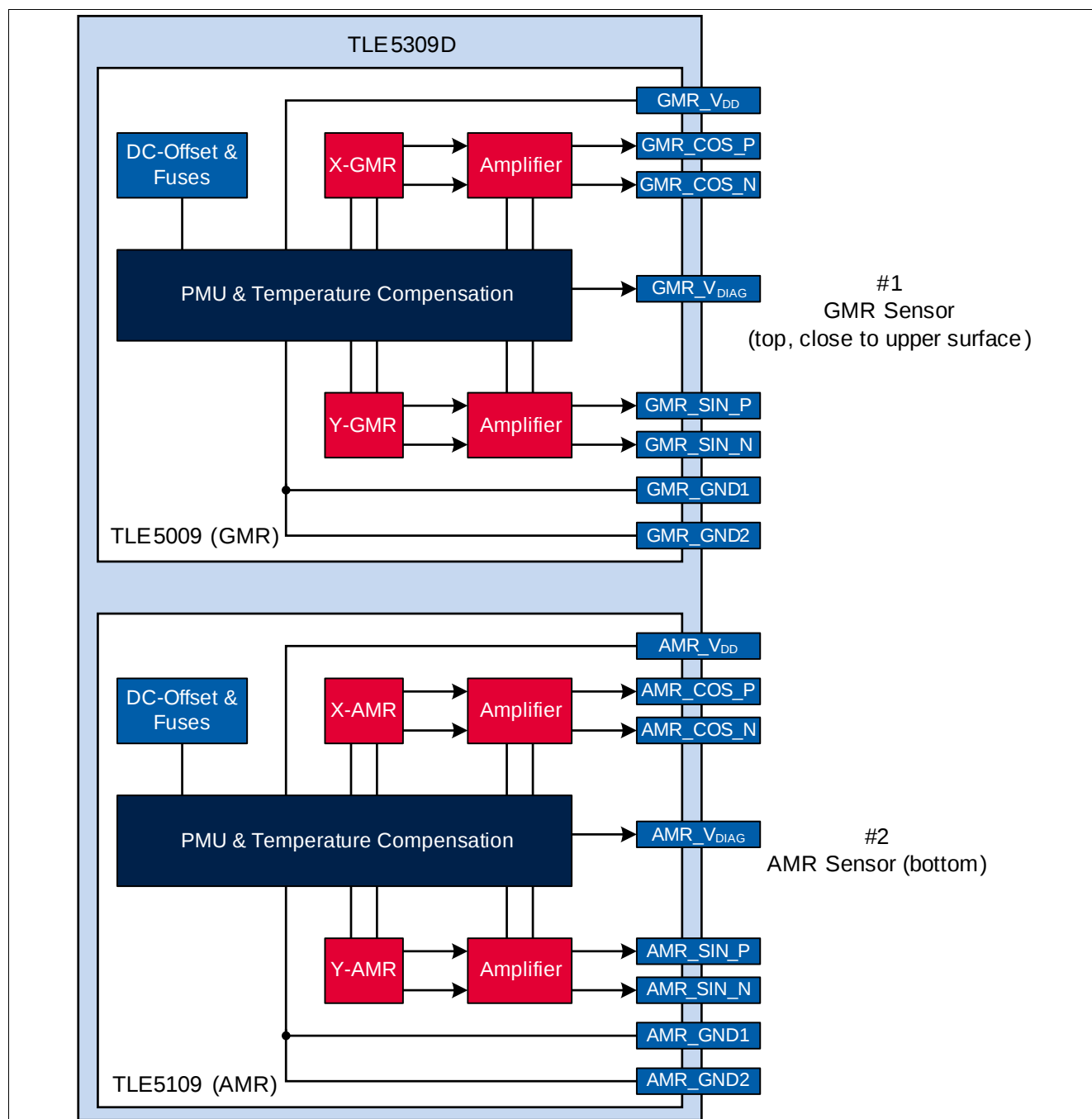
Figure 7 TLE5309D block diagram
