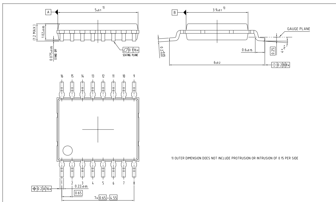
Figure 21 Package dimensions
