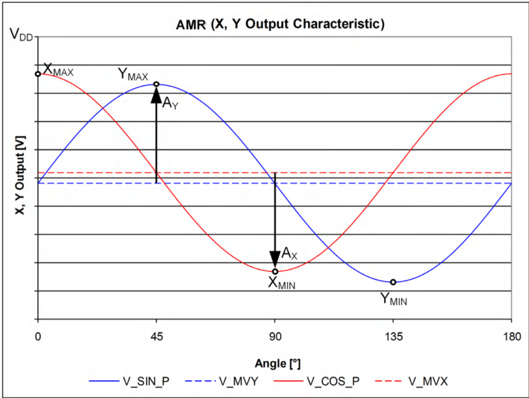
Figure 16 AMR sensor single-ended output signals
