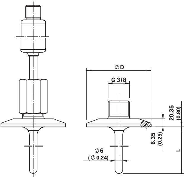
Complete assembly
