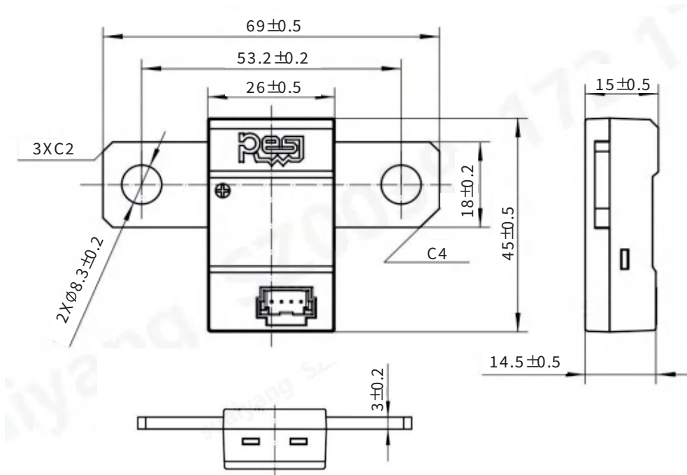
Figure 8.1 Structure Diagram
