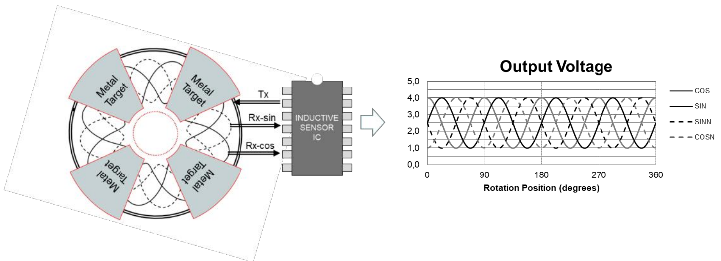
Figure 31. Coil Design and Signal Output for a 4 \times 90^\circ Rotary Sensor
