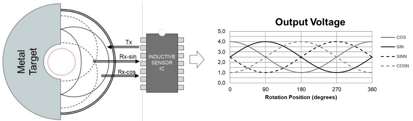
Figure 28. Coil Design and Signal Output for a 360^\circ Rotary Sensor
