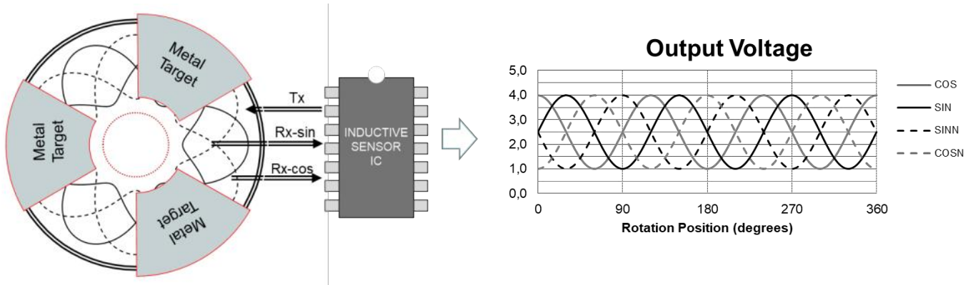
Figure 30. Coil Design and Signal Output for a 3 \times 120^\circ Rotary Sensor
