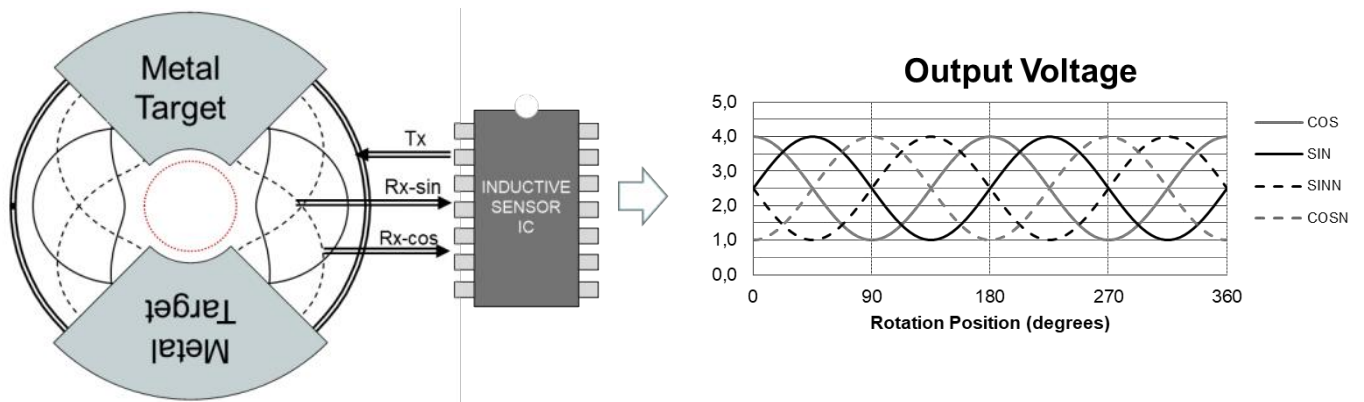
Figure 29. Coil Design and Signal Output for a 2 \times 180^\circ Rotary Sensor
