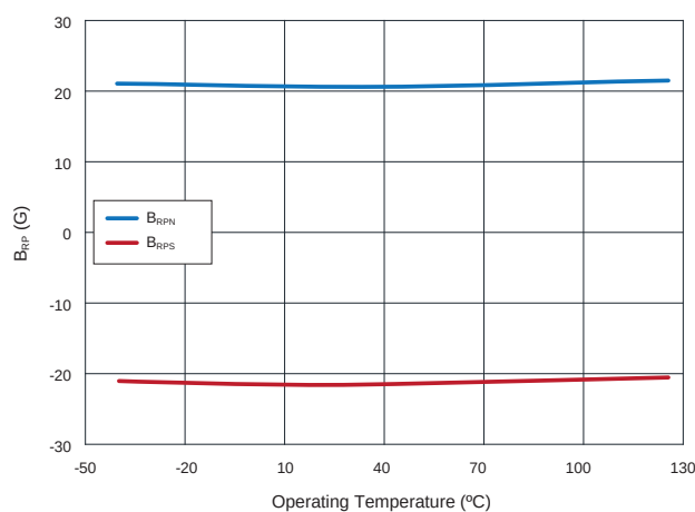
12.7 RR122-1B12-511 / 512 B_{RPN} (Blue) and B_{RPS} (Red) vs. Operating Temperature at V_{DD}=3.0 V
