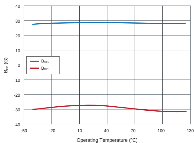
12.6 RR122-1B12-511 / 512 B_{OPN} (Blue) and B_{OPS} (Red) vs. Operating Temperature at V_{DD}=3.0 V
