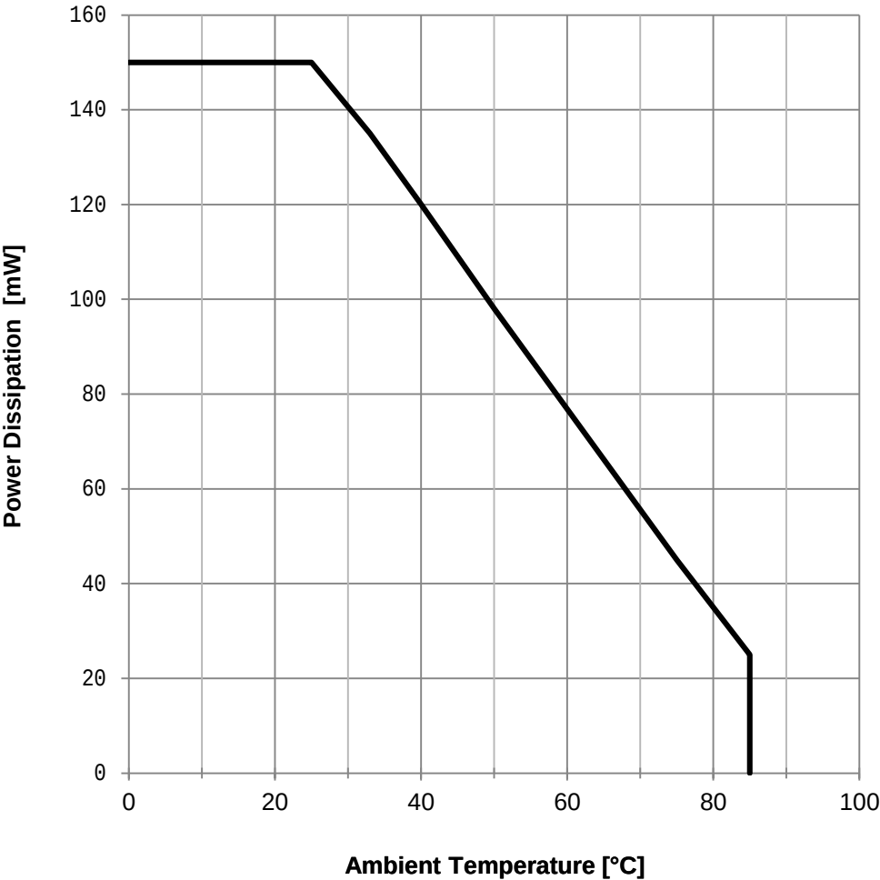
Derating Curve:
