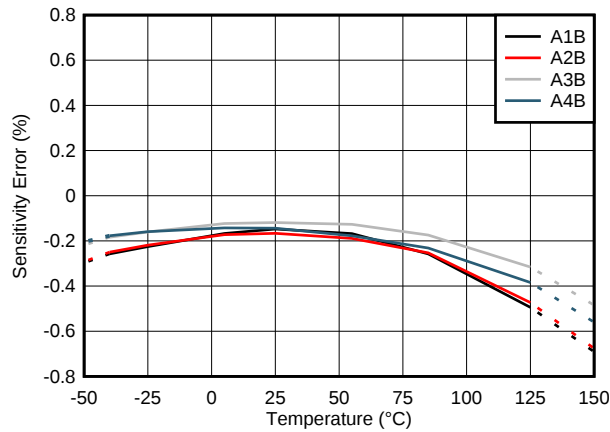
Figure 7-1. TMCS1101AxB Sensitivity Error vs Temperature
