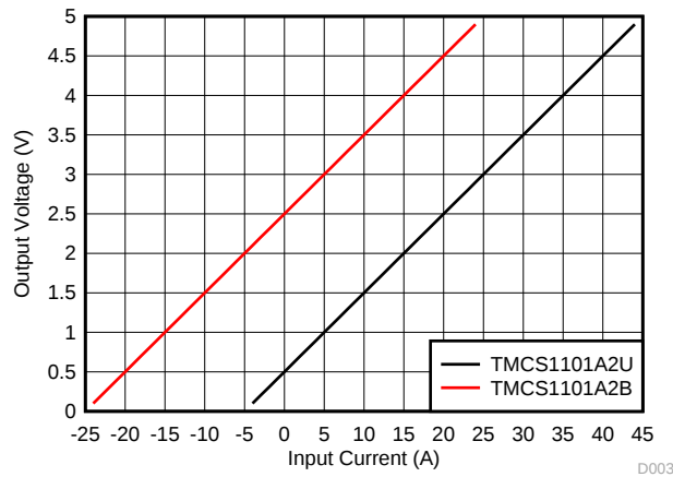
Figure 9-14. Output Voltage Relationship to Input Current for TMCS1101A2B and TMCS1101A2U
