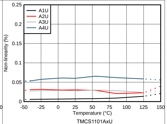
Figure 7-6. Non-Linearity vs. Temperature
