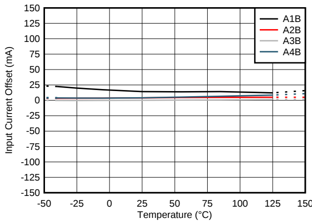
Figure 7-3. TMCS1101AxB Input Offset Current vs Temperature
