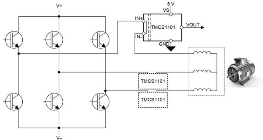
Figure 10-2. Inline Motor Phase Current Sensing
