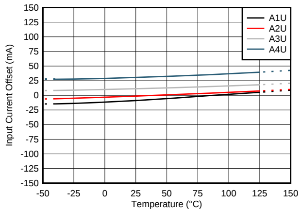
Figure 7-4. TMCS1101AxU Input Offset Current vs Temperature
