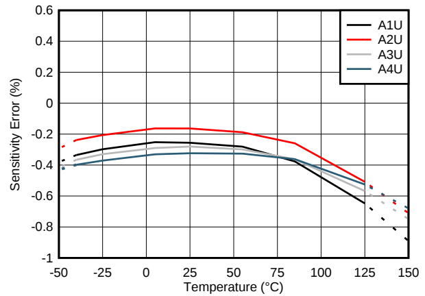
Figure 7-2. TMCS1101AxU Sensitivity Error vs Temperature
