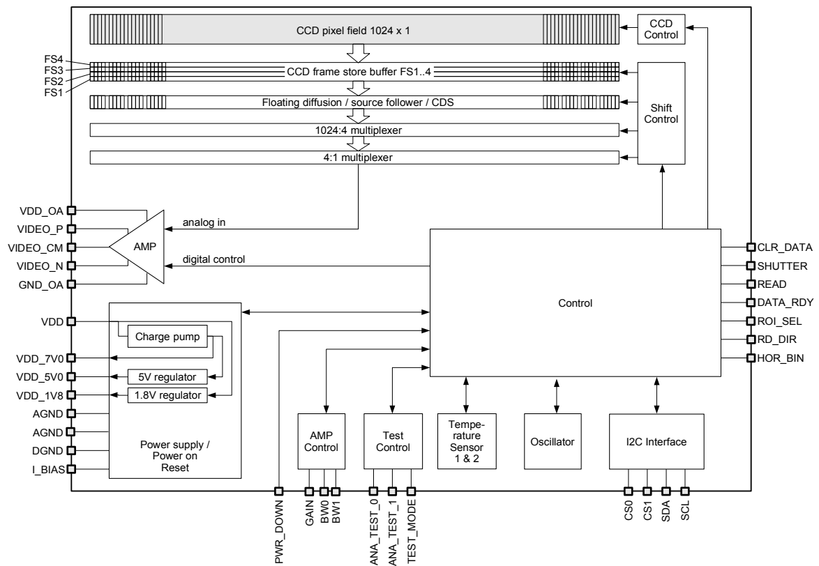
Figure 3: Block diagram
