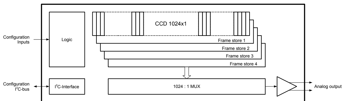
Figure 2: Block diagram
