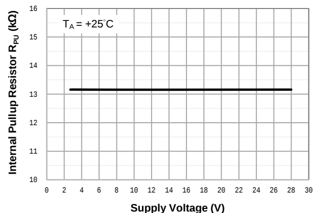
Internal Output Pullup Resistor vs. Supply Voltage
