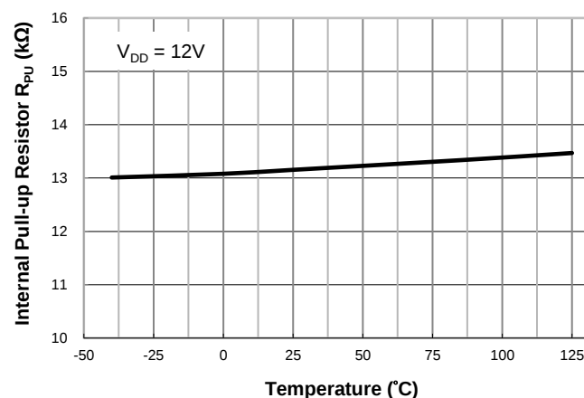
Internal Output Pullup Resistor vs. Temperature
