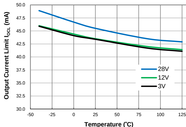
Output Current Limit vs. Temperature
