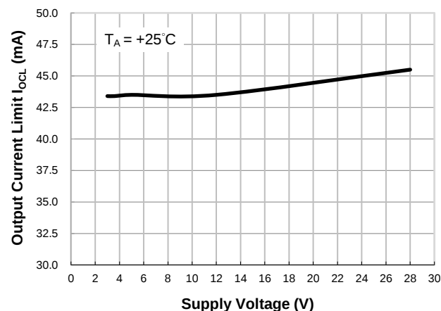
Output Current Limit vs. Supply Voltage
