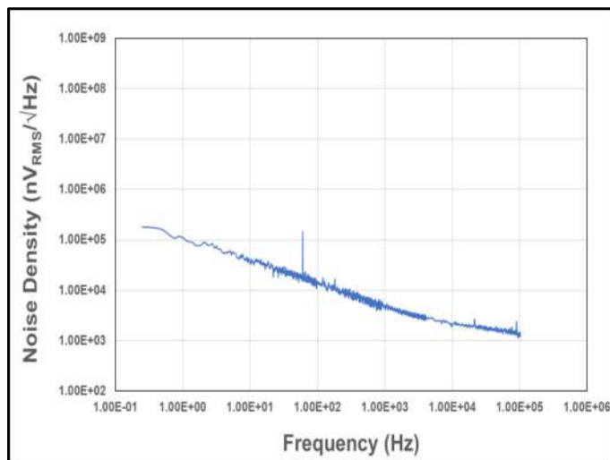
Figure 17. Noise Density vs. Frequency
