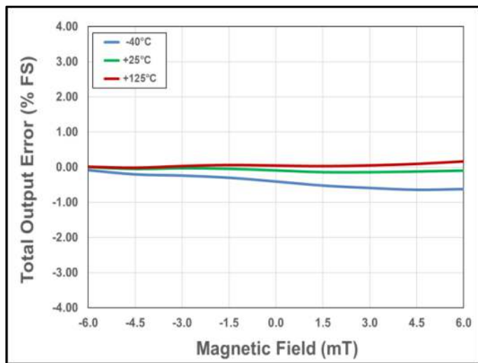
Figure 16. Total Output Error vs. B Field vs. Temperature
