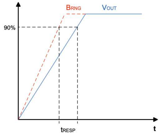
Figure 29. CT450 Response Time Curve
