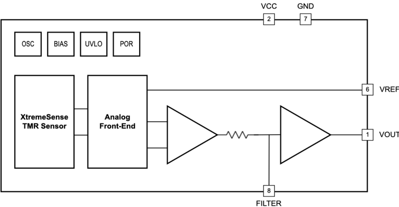
Figure 2. CT450 Functional Block Diagram for TSSOP-8
