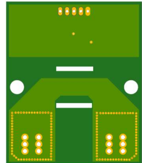
Figure 33. CTD450 Evaluation Board PCB Layout
