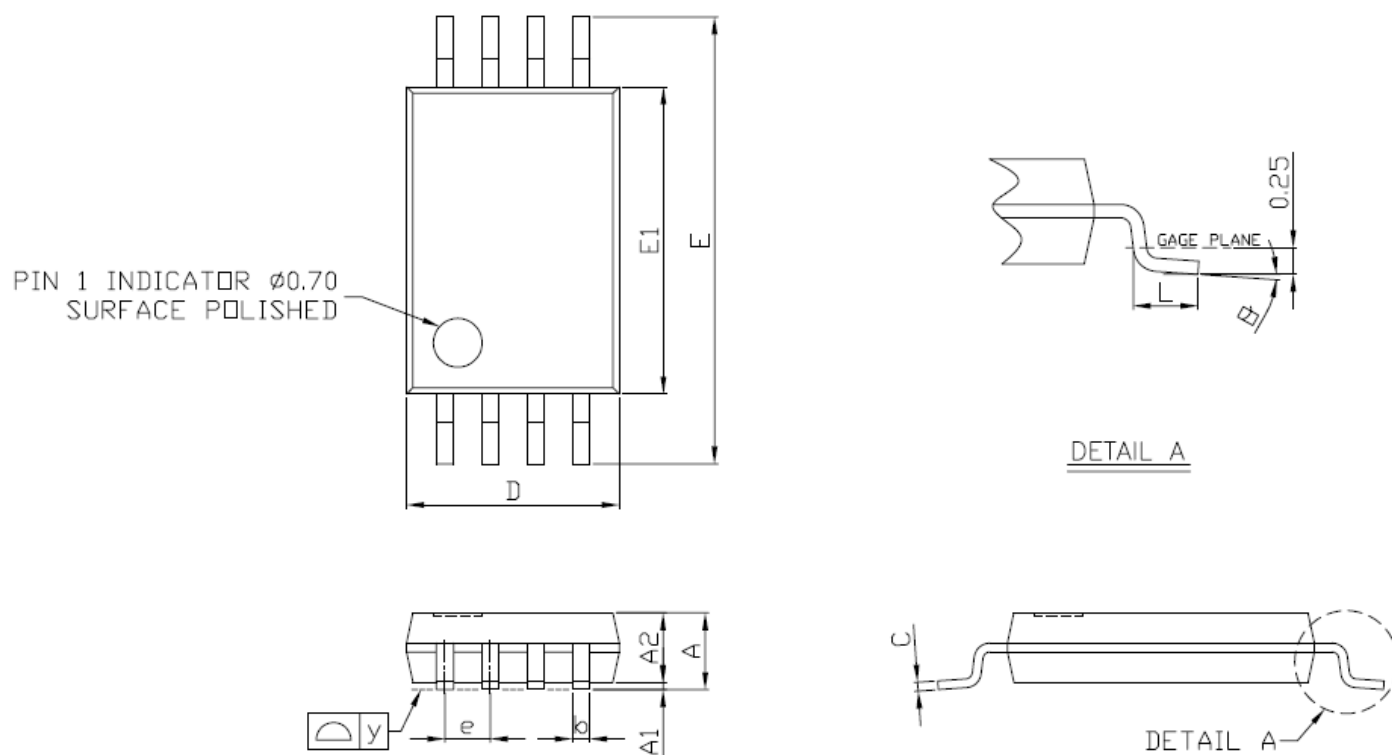
Figure 40. TSSOP-8 Package Drawing
