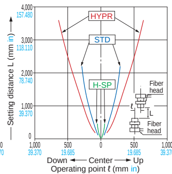
FT-R42W Thru-beam type
