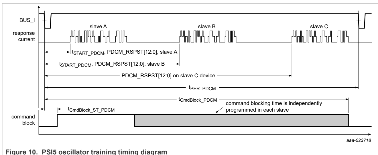
Figure 10. PSI5 oscillator training timing diagram
