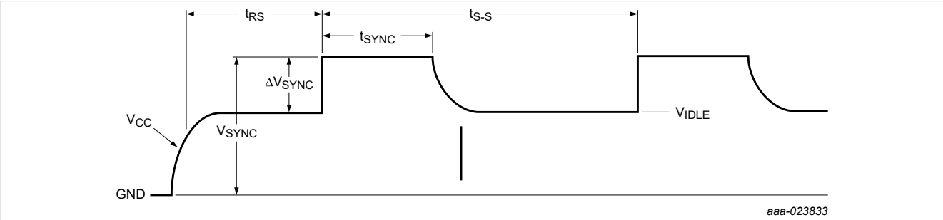
Figure 50. Sync pulse characteristics
