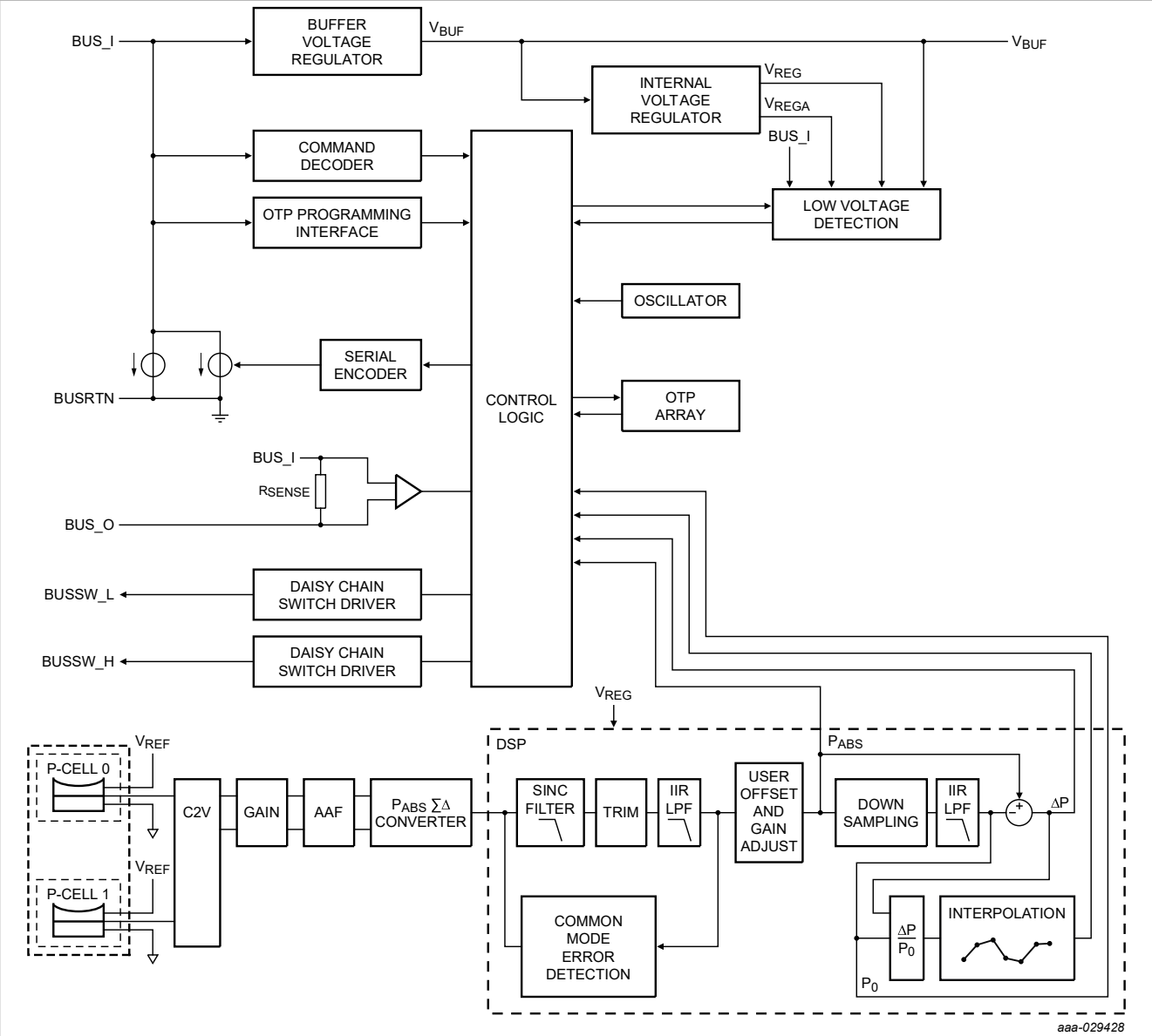
Figure 1. Block diagram
