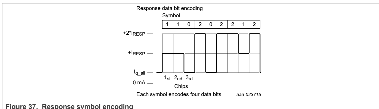
Figure 37. Response symbol encoding
