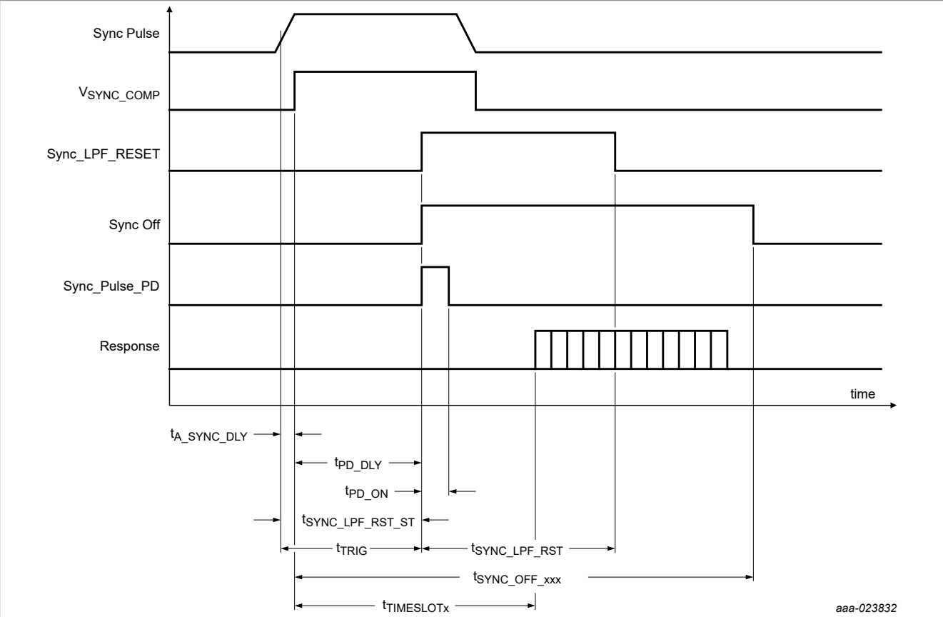
Figure 49. Synchronization pulse detection timing
