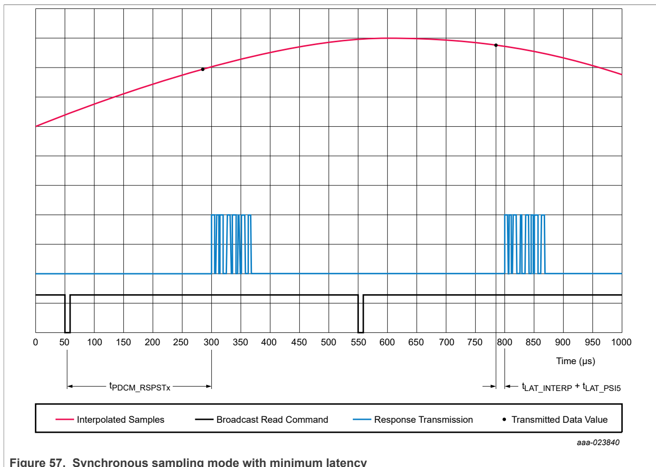
Figure 57. Synchronous sampling mode with minimum latency
