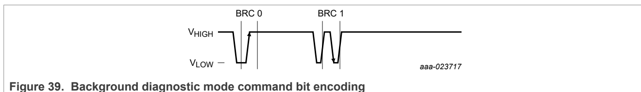
Figure 39. Background diagnostic mode command bit encoding
