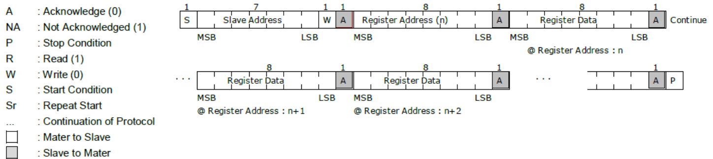
Figure 2. I 2 C Write-Register-Data Protocol
