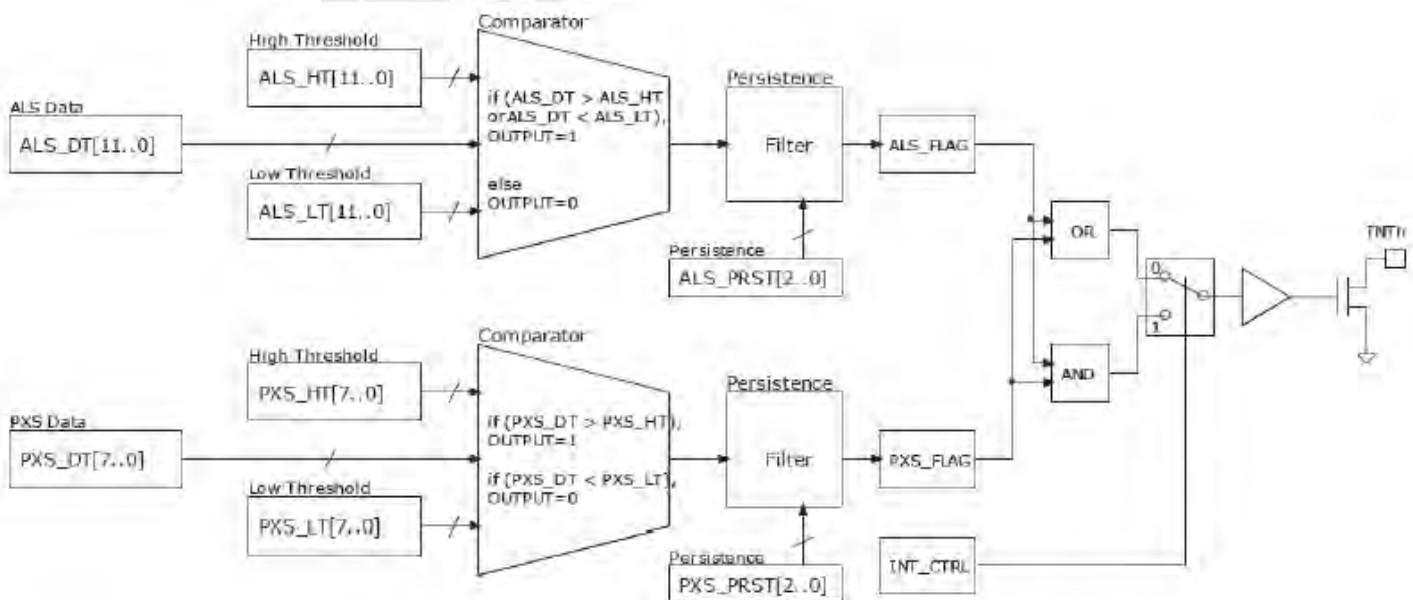
Figure 6. Interrupt operation
