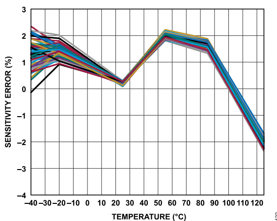
Figure 27. Sensitivity Error vs. Temperature, B_{SENSE} = 4 mT, G = 80 , V_{SET} = V_{DD} = 5 V
