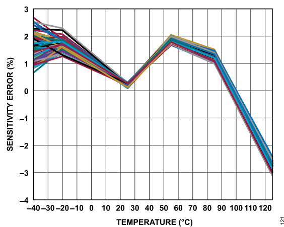
Figure 26. Sensitivity Error vs. Temperature, B_{SENSE} = 8 mT, G = 80 , V_{SET} = V_{DD} = 5 V
