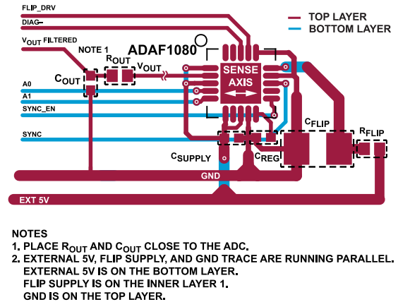
Figure 62. Recommended Layout for 2-Layer PCB
