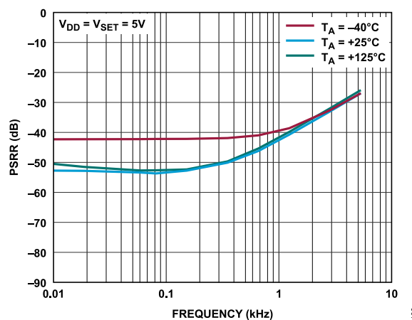
Figure 40. PSRR vs. Frequency, B_{\text{SENSE}} = 8 \text{ mT}
