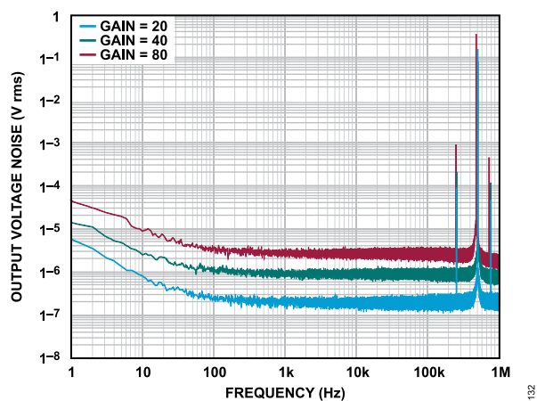
Figure 37. Output Voltage Noise vs. Frequency, External Chopping, f_{\text{SYNC}} = 1.6 \text{ MHz} , All Gain Settings
