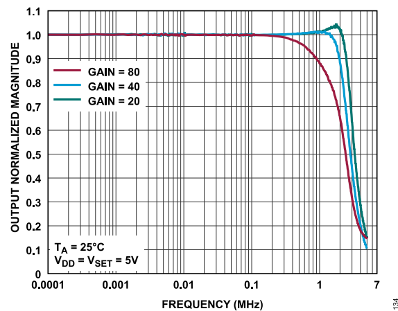
Figure 38. Output Normalized Magnitude vs. Frequency, V_{\text{SET}} = V_{\text{DD}} = 5 \text{ V} , T_A = 25^\circ\text{C}
