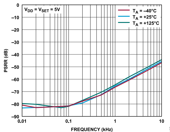
Figure 39. PSRR vs. Frequency, B_{\text{SENSE}} = 0 \text{ mT}
