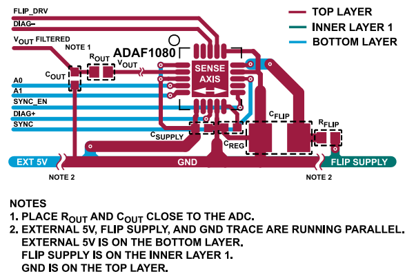
Figure 63. Recommended Layout for a 3-Layer PCB
