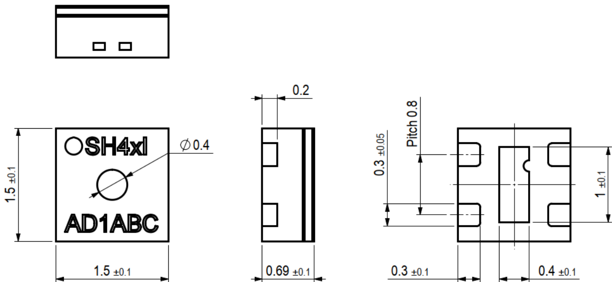
Figure 10. Dimensional drawing of SHT4xI-Digital with filter membrane including package tolerances (units mm)
