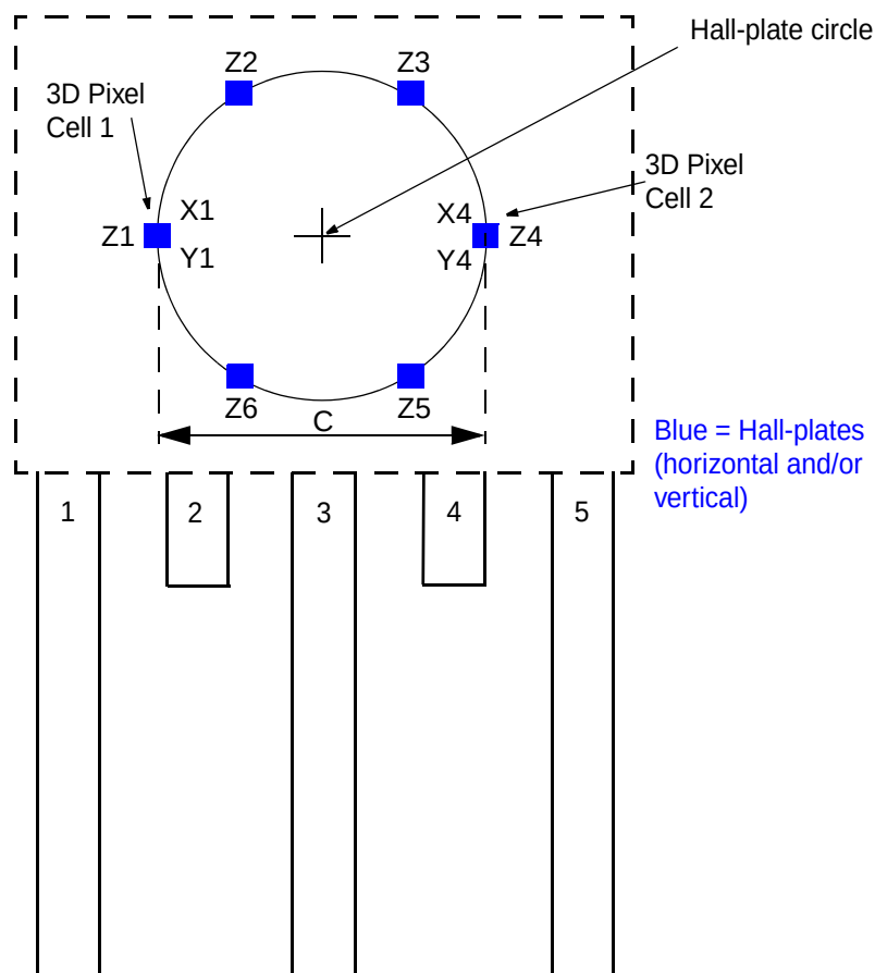
Fig. 5–3: Hall-plate configuration
