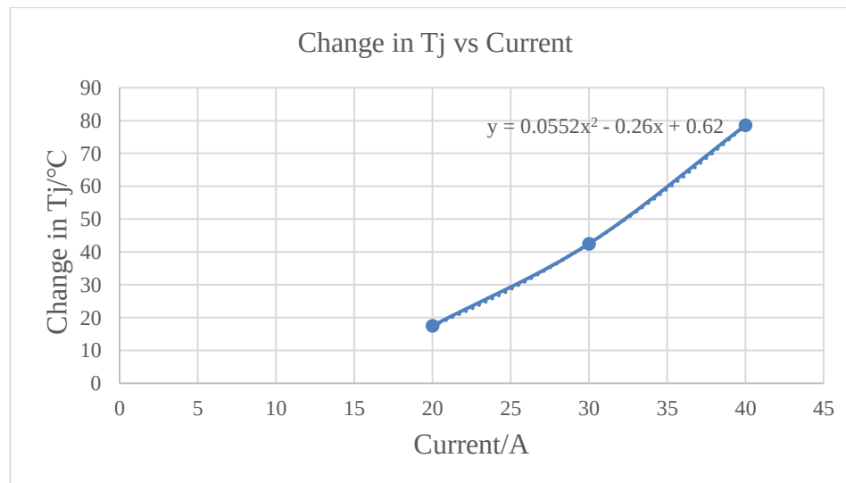
Figure 6.4 NSM2011 Estimation function of junction temperature at different currents (PCB is in worst case)
