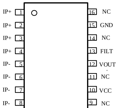
Figure 1.1 NSM2011 Package
