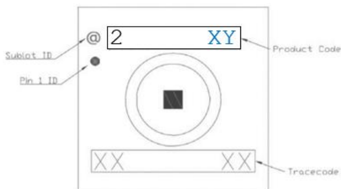
Figure 20: ENS21x marking
