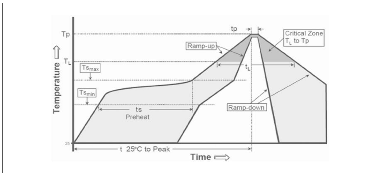
Figure 17: Soldering recommendations
