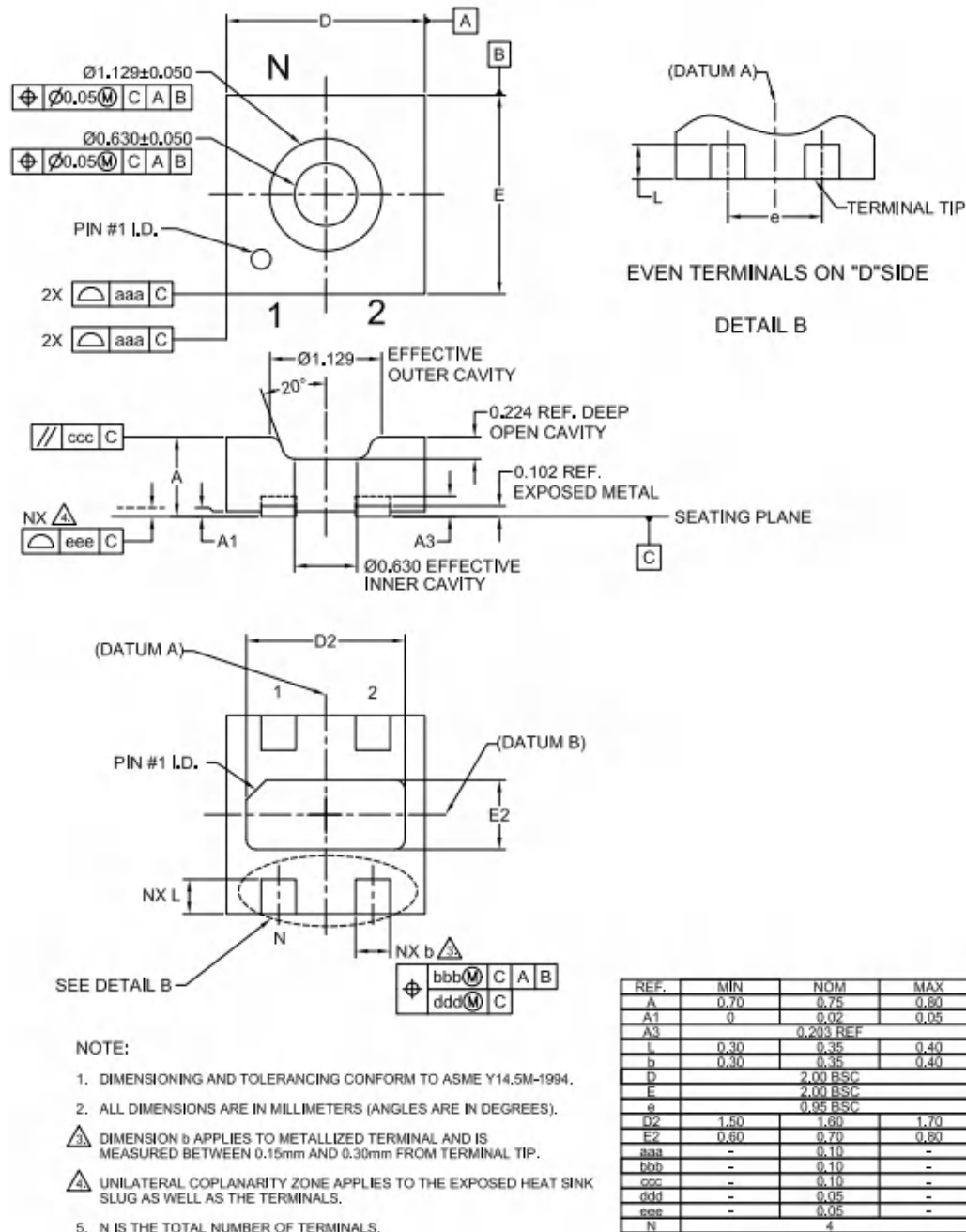
Figure 19: Package outline
