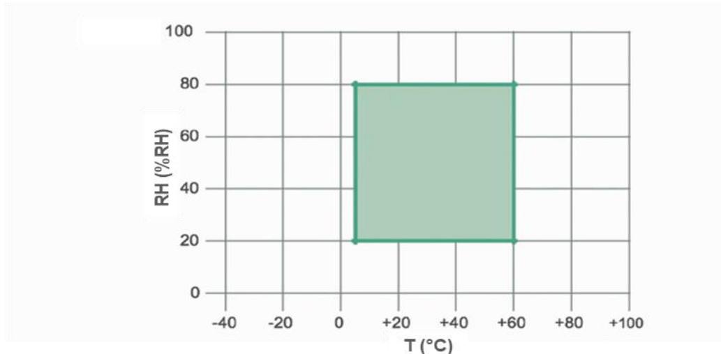
Figure 16: Recommended operating conditions
