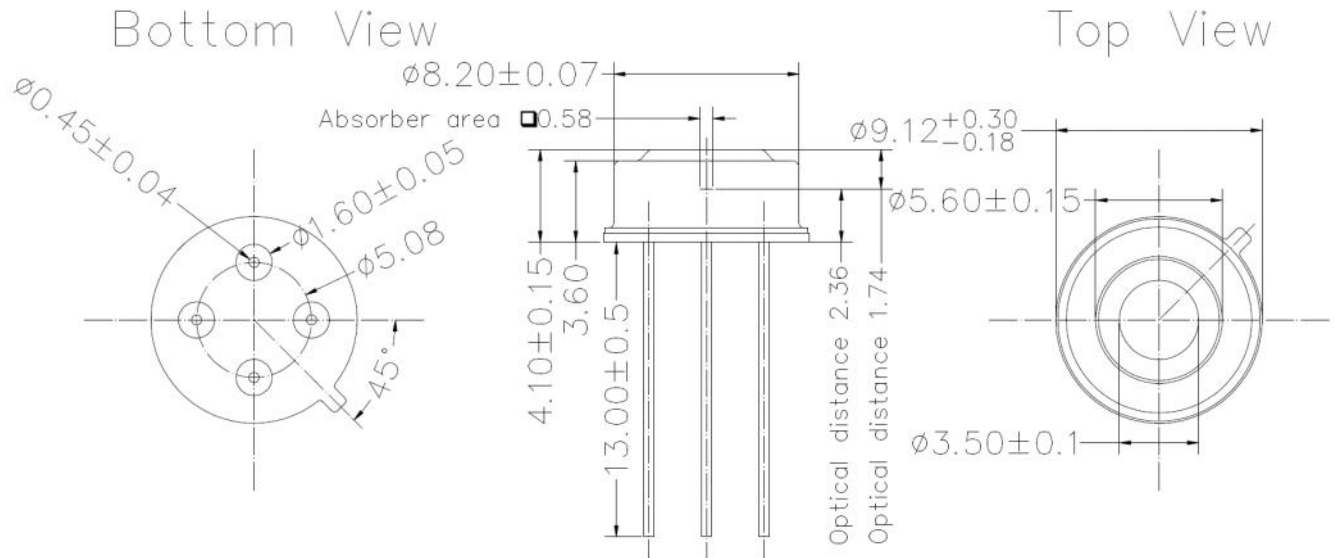
Figure 43: MLX90614xxA package
