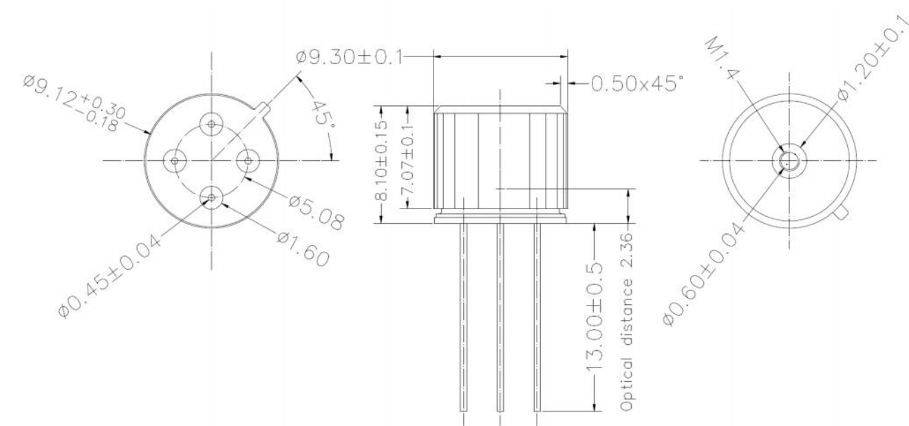
Figure 48 MLX90614xCK package
