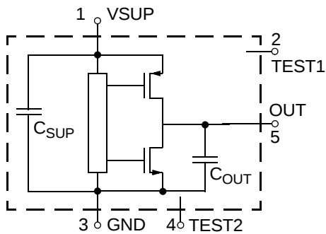
Fig. 4–3: Pin configuration
