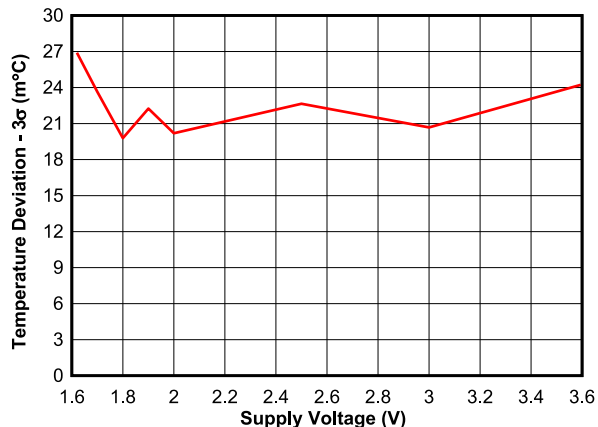
Figure 6-9. Supply Sensitivity- Temperature Measurement Accuracy
