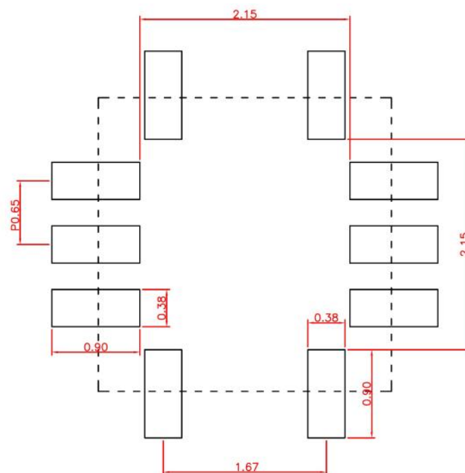
Figure 11.2 Pad Dimensions
