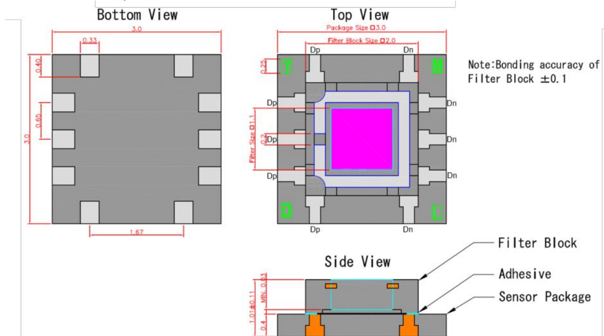
Figure 11.1 Outline Dimensions
