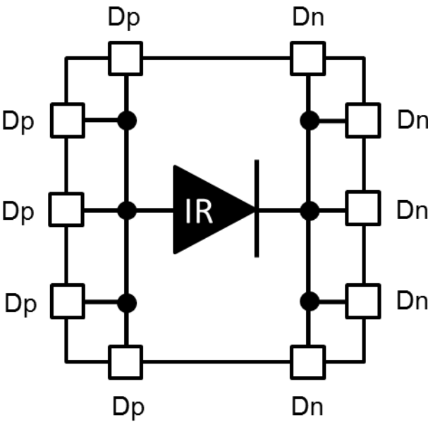
Figure 4.1 Block Diagram
