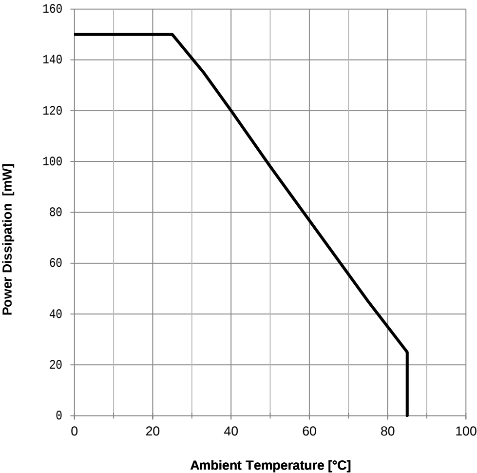
Derating Curve:
