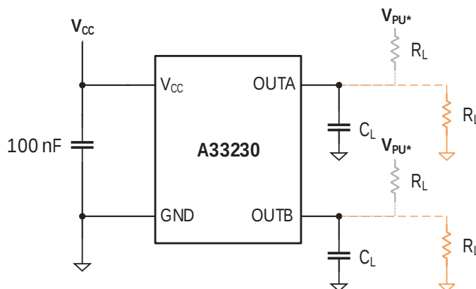
Figure 2: Typical Application Circuit
