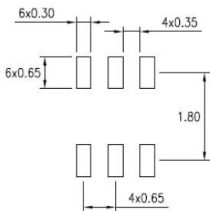
Recommended Land Pattern for LTR-381RGB-ALI
