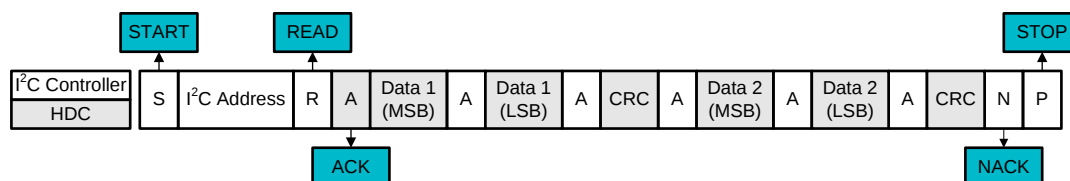
Figure 8-8. I²C Read Multi Data Result, Final CRC Retained
