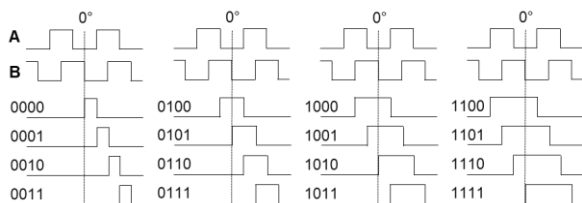
Figure 17: ILIP Parameter Effect on Index Shape
