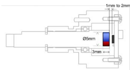
Figure 5: Potentiometer-Like Assembly
