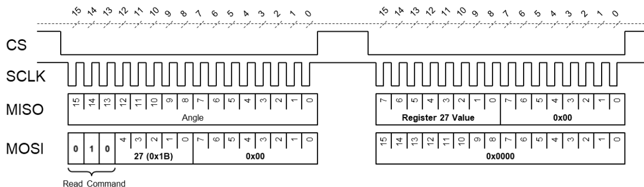
Figure 12: Example Read Magnetic Level Flags High and Low (MGH, MGL) on Register 27, Bits[7:6]
