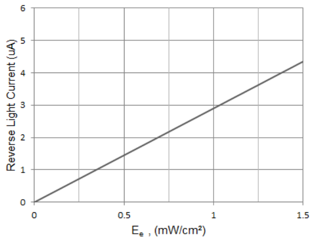
Reverse Light Current VS. E_e
