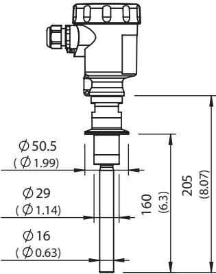
LBV311 threaded version Tri-Clamp
