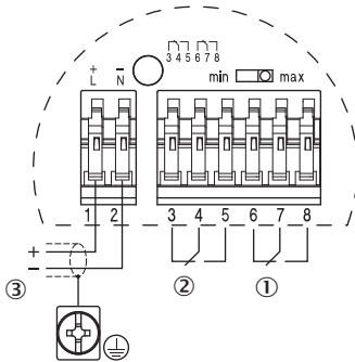
Double relay connection diagram
